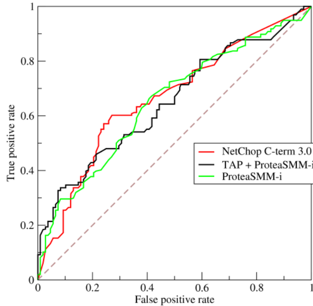
Figure 1: An example ROC curve, care of Wikipedia
